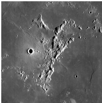
Montes Riphæus, LRO (Lunar Reconnaissance Orbiter) via wikipedia
